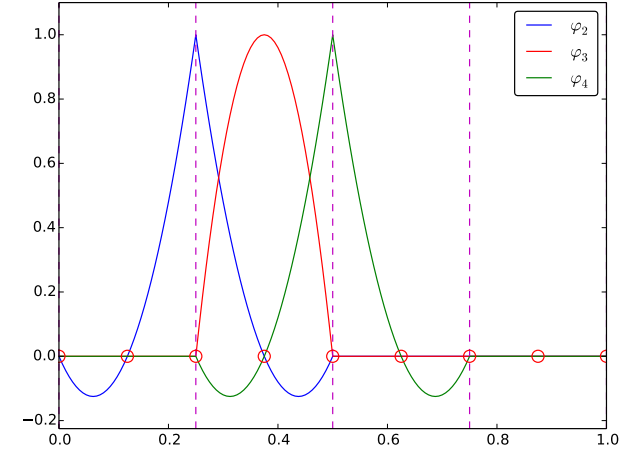
Figure 20: Illustration of the piecewise quadratic basis functions associated with nodes in an element.
