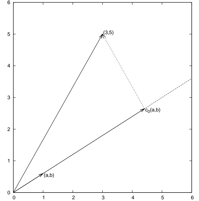
Figure 1: Approximation of a two-dimensional vector in a one-dimensional vector space.
