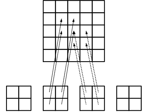
Figure 28: Illustration of matrix assembly: regularly numbered P1 elements.
