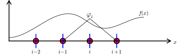
Figure 26: Right-hand side integral with the product of a basis function and the given function to approximate.
