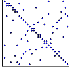
Figure 32: Matrix sparsity pattern for left-to-right numbering (left) and random numbering (right) of nodes in P1 elements.
