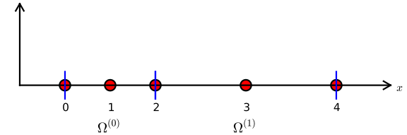
Figure 18: Finite element mesh with 2 elements and 5 nodes.
