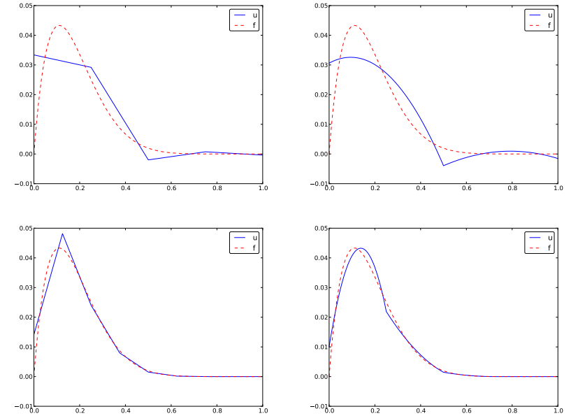
Figure 31: Comparison of the finite element approximations: 4 P1 elements with 5 nodes (upper left), 2 P2 elements with 5 nodes (upper right), 8 P1 elements with 9 nodes (lower left), and 4 P2 elements with 9 nodes (lower right).
