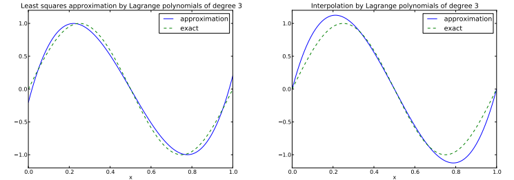
Figure 10: Approximation via least squares (left) and interpolation (right) of a sine function by Lagrange interpolating polynomials of degree 3.
