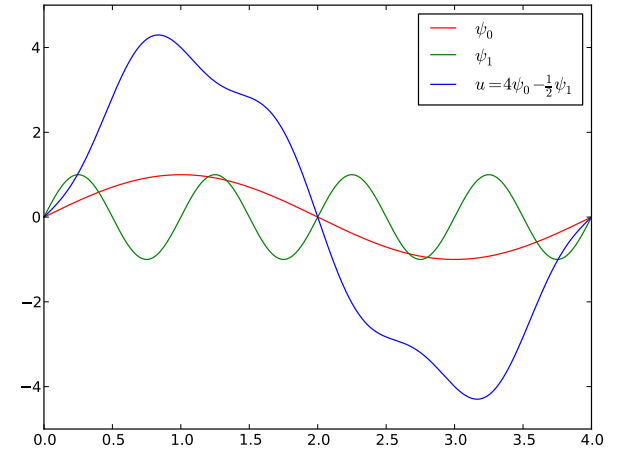
Figure 15: A function resulting from a weighted sum of two sine basis functions.
