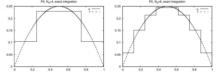
Figure 34: Approximation of a parabola by 4 (left) and 8 (right) P0 elements.
