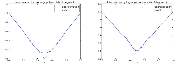
Figure 13: Interpolation of an absolute value function by Lagrange polynomials and Chebyshev nodes as interpolation points: degree 7 (left) and 14 (right).
