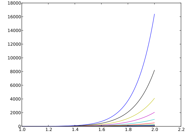
Figure 3: The 15 first basis functions x^i , i = 0, \dots, 14 .
