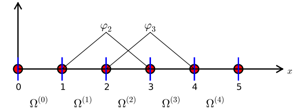
Figure 24: Illustration of the piecewise linear basis functions corresponding to global node 2 and 3.
