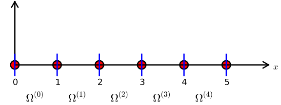
Figure 17: Finite element mesh with 5 elements and 6 nodes.
