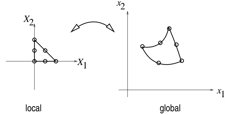
Figure 47: Isoparametric mapping of a P2 element.
