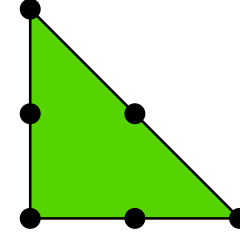
Figure 42: 2D P2 element.
