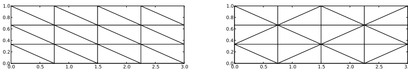
Fig. 3.21 Example on 2D P1 elements.
