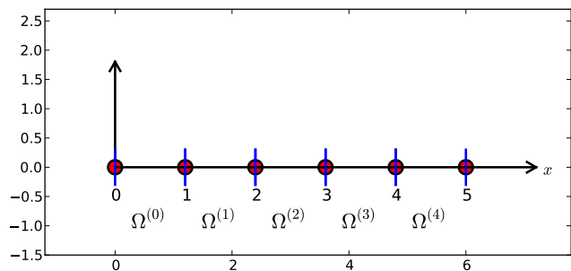
Figure 15: Finite element mesh with 5 elements and 6 nodes.
