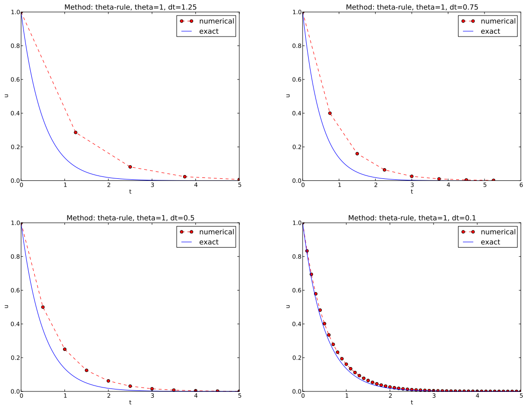
Figure 15: Backward Euler.
