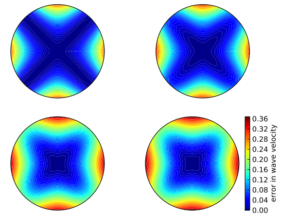
Figure 7: Error in numerical dispersion in 2D.
