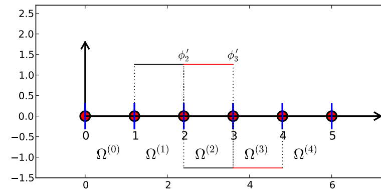
Figure 47: Illustration of the derivative of piecewise linear basis functions associated with nodes in cell 2.
