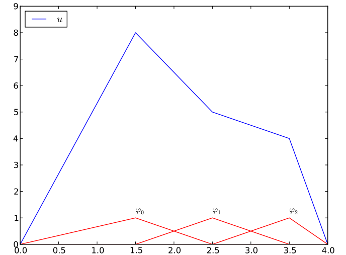
Figure 14: A function resulting from adding three local piecewise linear functions.
