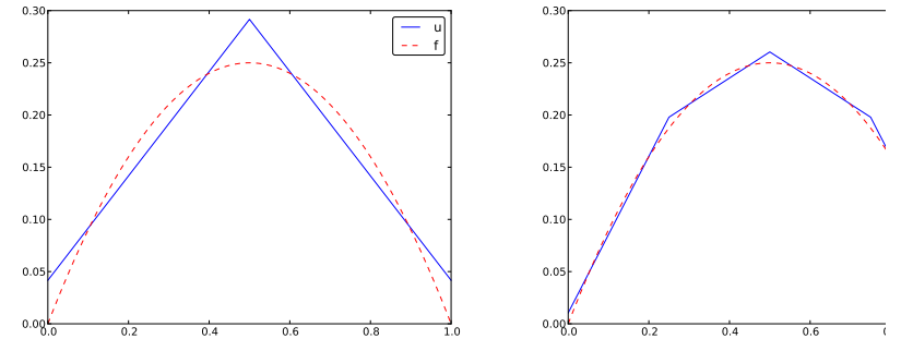
Figure 25: Least squares approximation of a parabola using 2 (left) (right) P1 elements.
