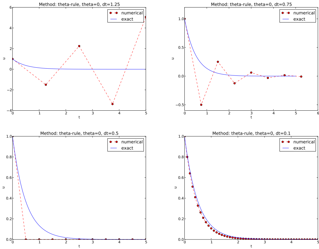
Figure 11: Forward Euler.
