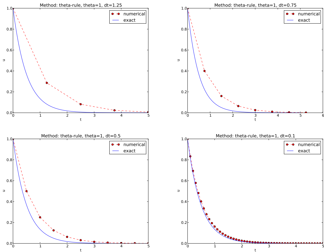
Figure 9: Backward Euler.
