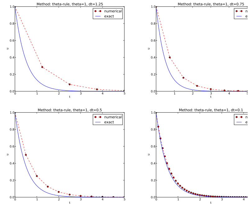
Figure 9: Backward Euler.
