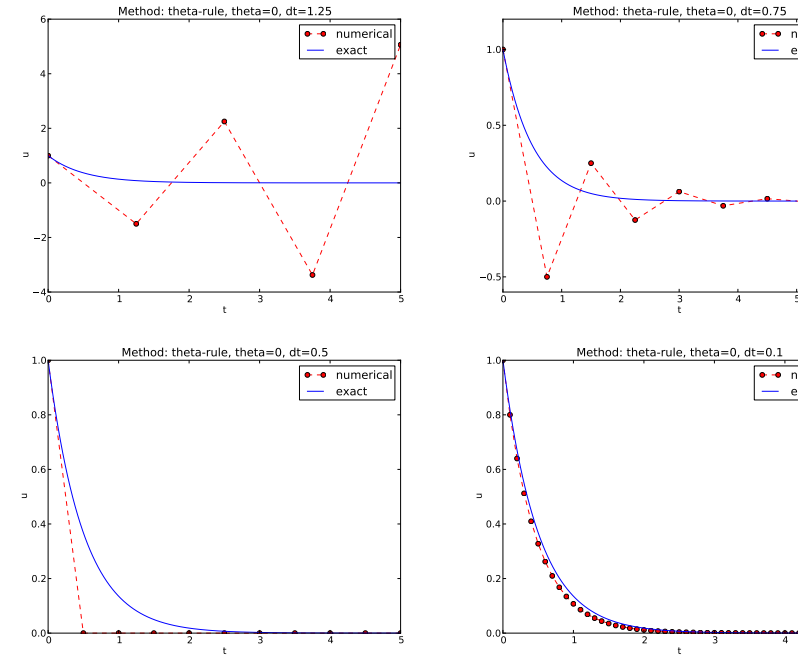
Figure 11: Forward Euler.
